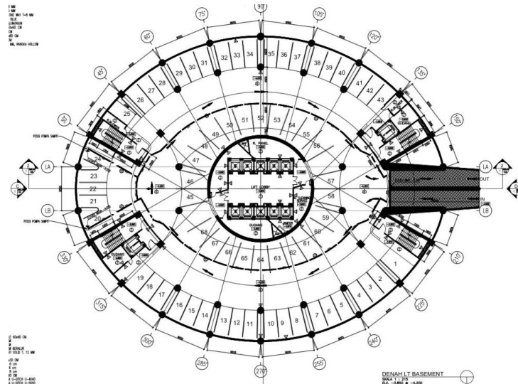
Gambar 1. 1 Denah Lahan Parkir Basemen TULT
