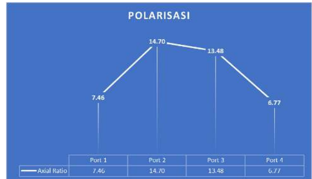
GAMBAR 4 Axial Ratio Pengukuran
