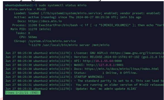
Gambar 3. 6 Status tools MinIO
