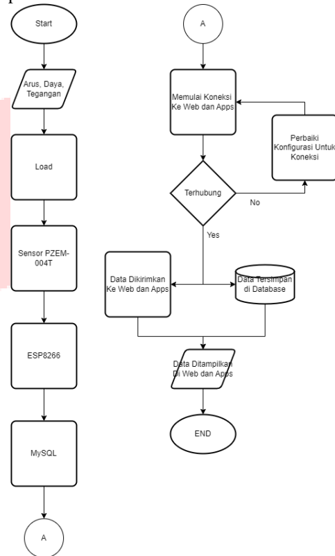
Gambar 3.2 Diagram Alir
