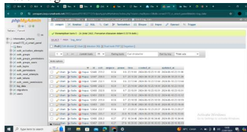
Gambar 4.2 PHPMyAdmin
