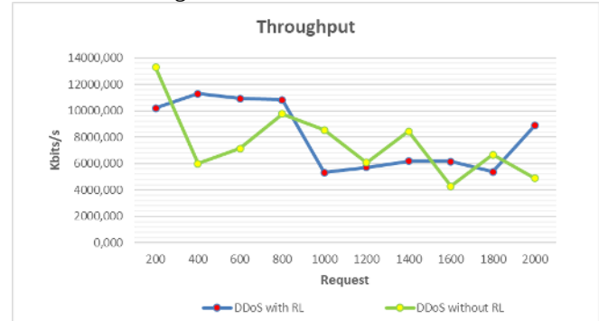
GAMBAR 4.1 Grafik Throughput
