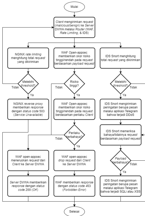
GAMBAR 3.2 Diagram Alir
