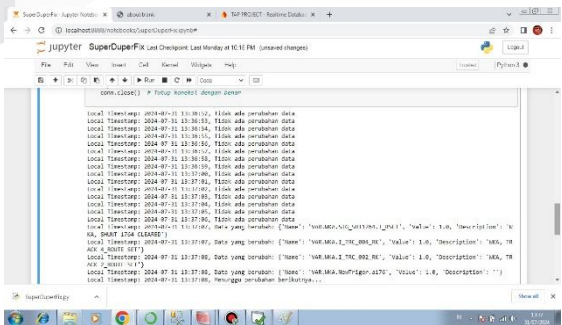
GAMBAR 4.3 Output Python
