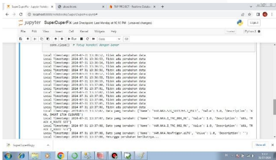
GAMBAR 4.1 Output Python
