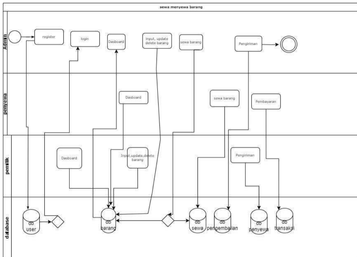
Gambar 5. proses BPMN
