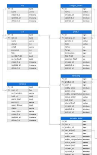
Gambar 3. Class Diagram
