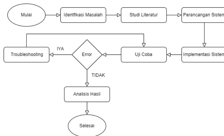
Gambar 3. 1. Diagram Alur
