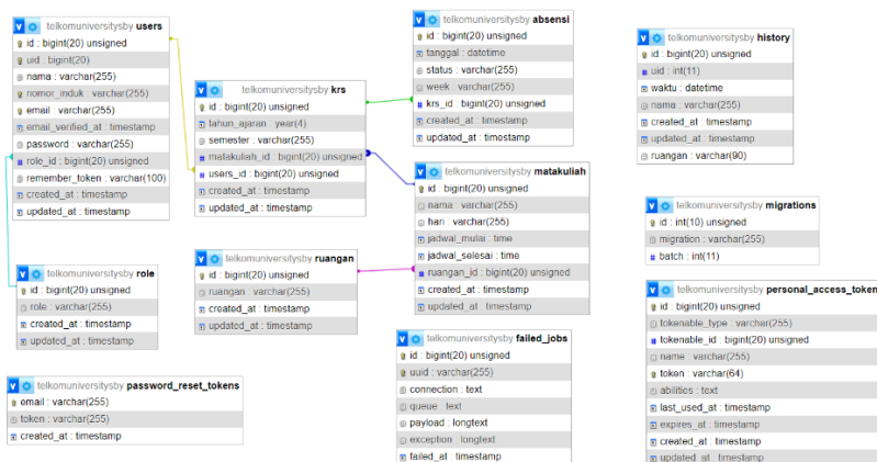
Gambar 3. 4. 2. 1 Implementasi Database
