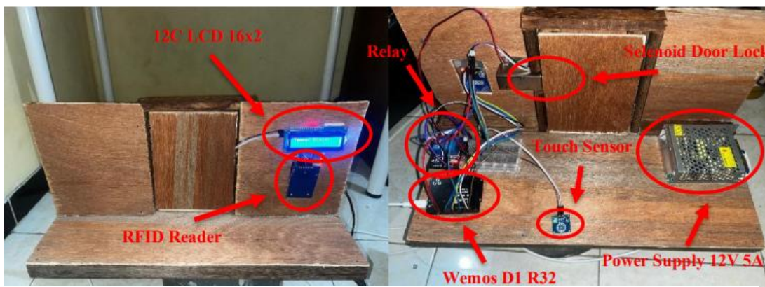
Gambar 3. 4. 1. 1. Implementasi Prototype
