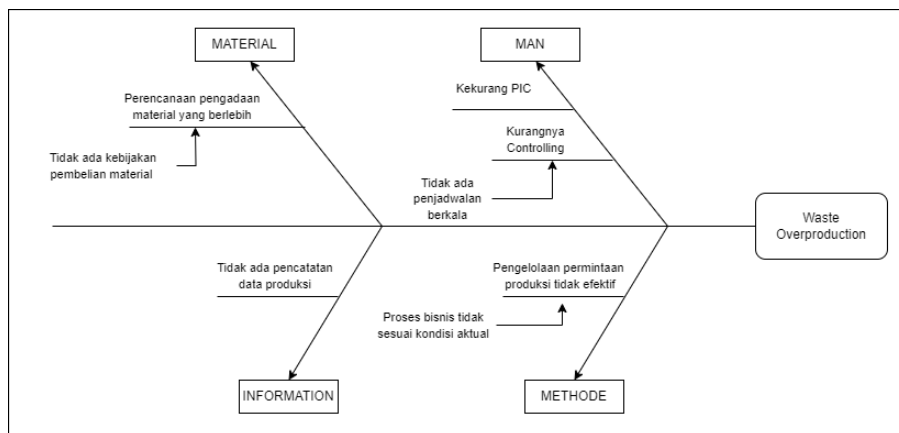
Gambar I. 1 Fishbone Diagram
