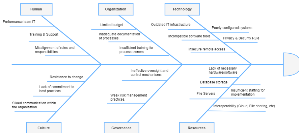
Gambar 1.1 Fishbone Diagram
