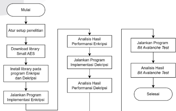
GAMBAR 5. Alur Implementasi Small AES
