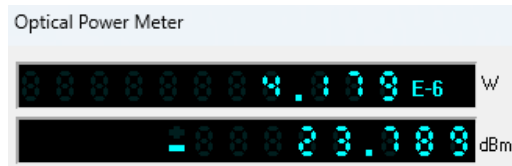
Gambar 10 Hasil Received Power Terburuk Pada Link Backhaul
