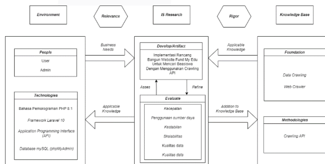
GAMBAR 2 Model Konseptual
