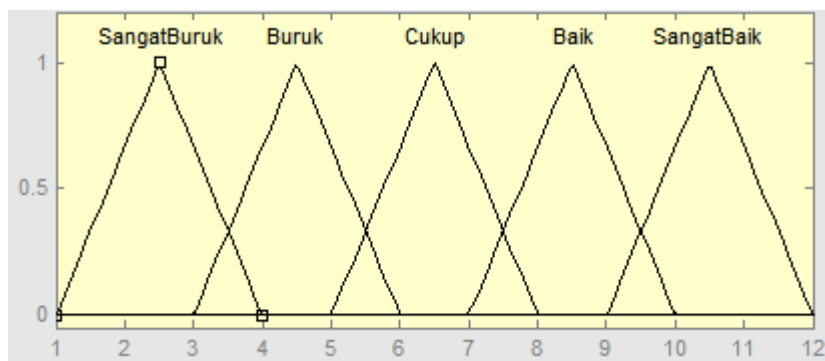
Gambar 2.1 Fuzzy Set
