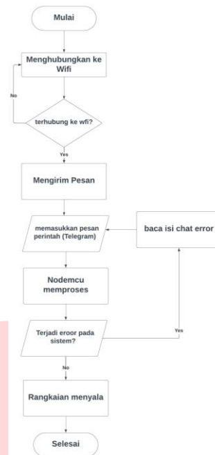
Gambar 2 Flowchart
