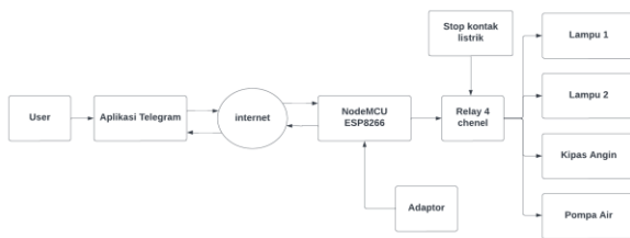
Gambar 5 Usecase Diagram
