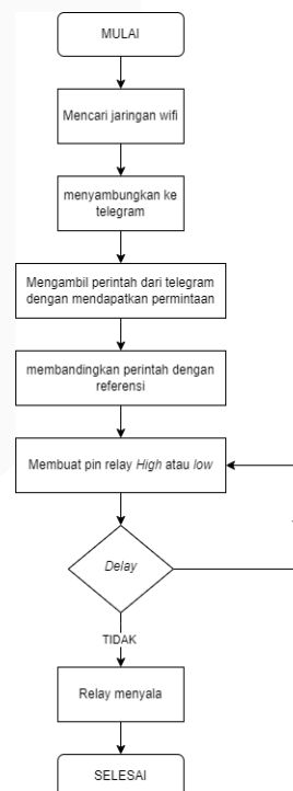
Gambar 3 Flowchart sistem kerja NodeMCU ESP8266
