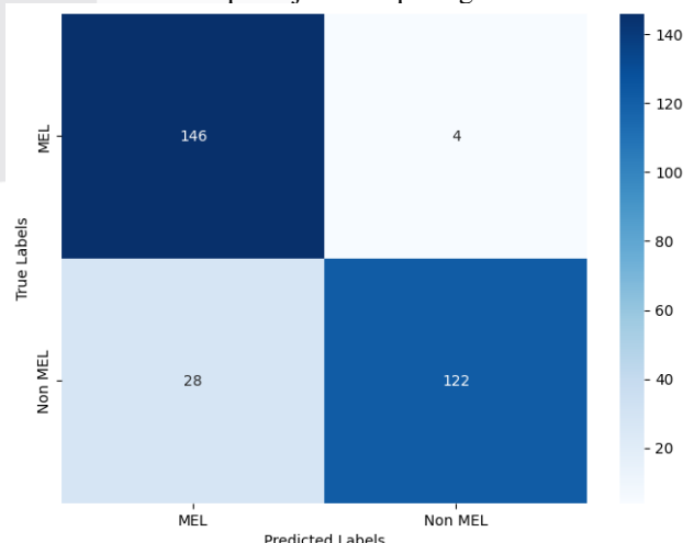
GAMBAR 4.2 Confusion Matrix
