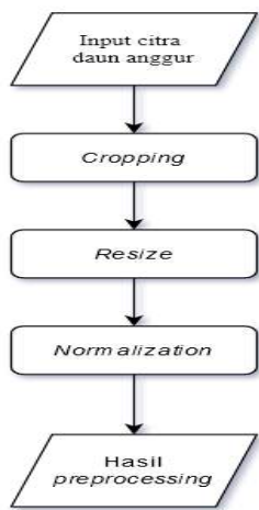
GAMBAR 7 Tahap preprocessing.
