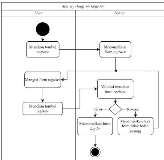
GAMBAR 3 Activity Diagram 2
