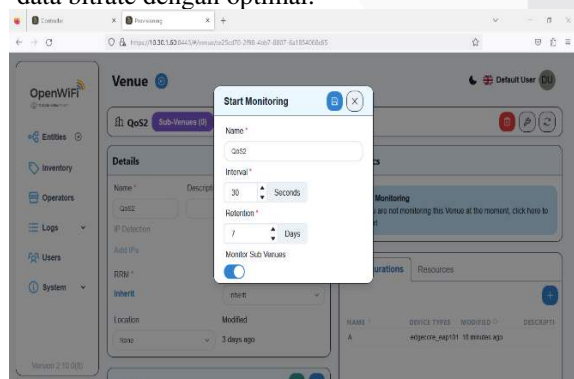
GAMBAR 12. Menu Monitoring
