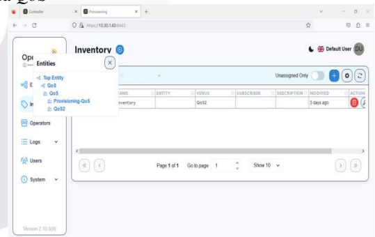
GAMBAR 3. Menu Entities
