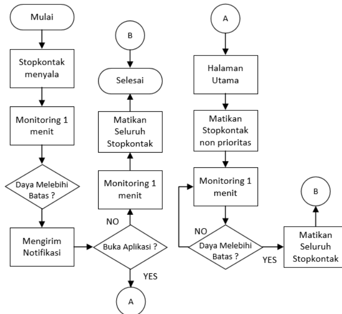
Gambar 1.3 Flowchart Stopkontak Non Prioritas
