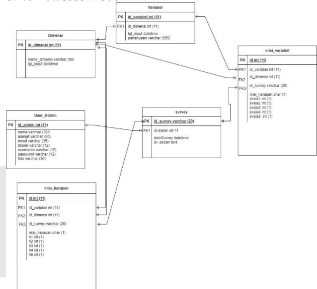
Gambar 3 Database Model
