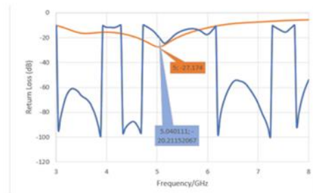
Gambar 4.5 Hasil Perbandingan Return Loss
