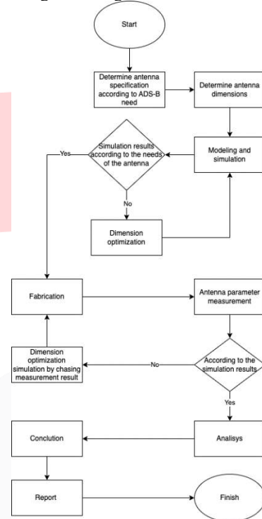
FIGURE 6 Antenna manufacturing
