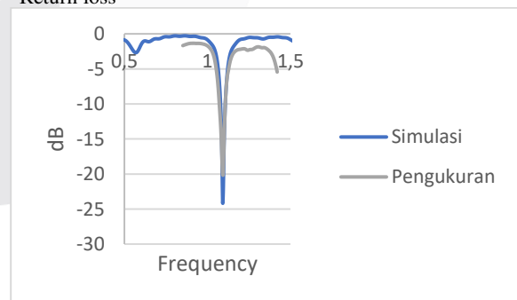
FIGURE 7 ADS-B antenna measurement results of S-Parameters
