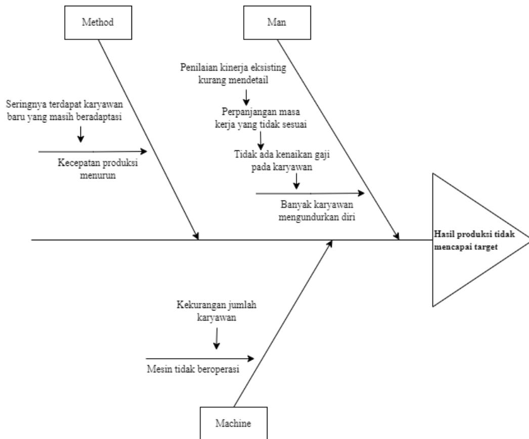
Gambar I. 3 Diagram Fishbone
