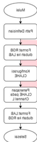
GAMBAR 6. Proses CLAHE
