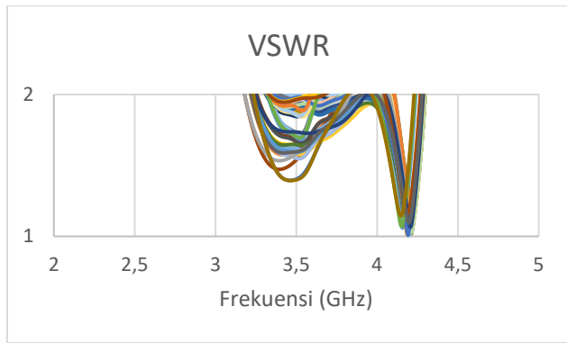
GAMBAR 7 VSWR Massive MIMO
