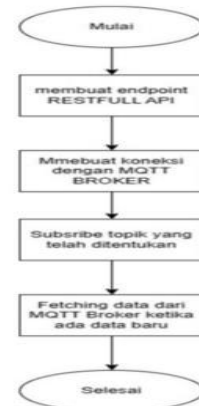
GAMBAR 3.7 Diagram Alir Backend
