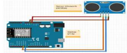
GAMBAR 3. 6 Prototype Rangkaian Sensor Ultrasonik
