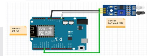
GAMBAR 3. 7 Prototype Rangkaian Sensor Infrared
