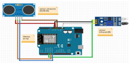
GAMBAR 3. 1 Prototype Rangkaian Wemos D1 R2
