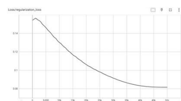
Gambar 12 Regularization loss.
