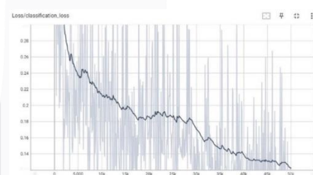
Gambar 10 Classification loss.
