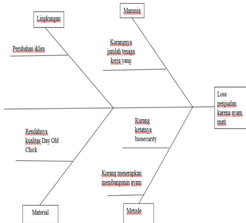
Gambar I.3 Diagram Fishbone
