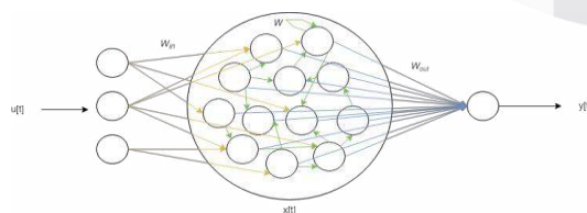
GAMBAR 1. Echo state network model
