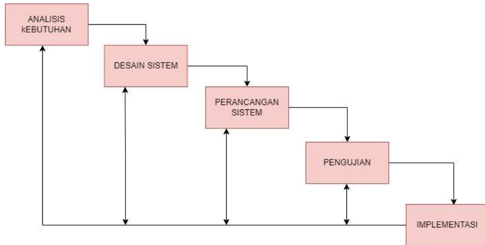
Gambar 1.1 Diagram Waterfall
