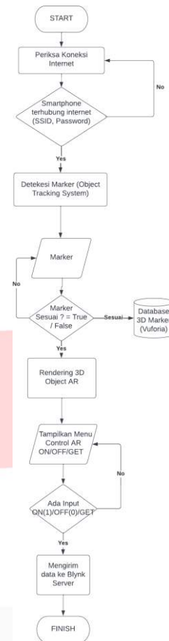
GAMBAR 2 (FLOWCHART SISTEM)
