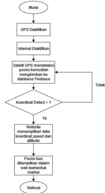
Gambar 2 Flowchart Program
