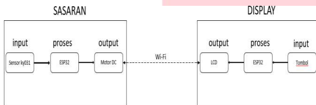
Gambar 2 Blok Diagram
