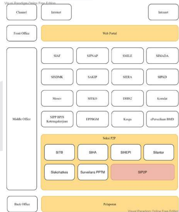
GAMBAR 2 SOLUTION CONCEPT DIAGRAM
