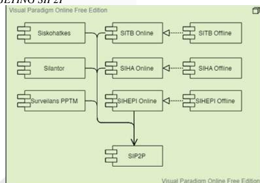
GAMBAR 7 TARGETING APPLICATION COMMUNICATION DIAGRAM
