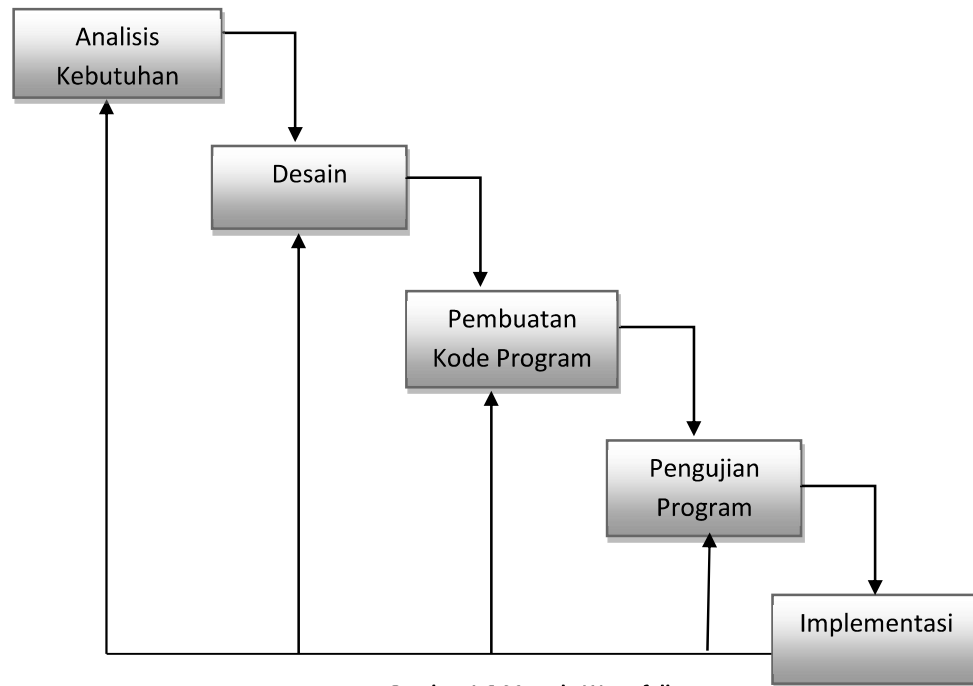
Gambar 1-3 Metode Waterfall
