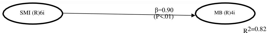
Gambar 4.3 Model Penelitian
