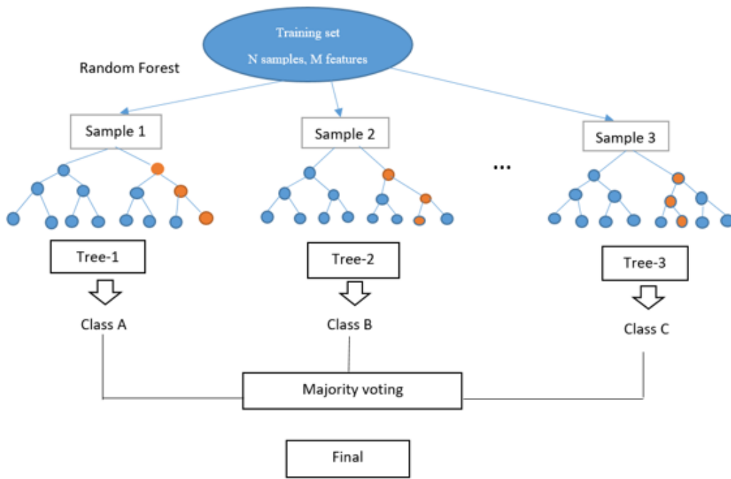
Random Forest Simplified
