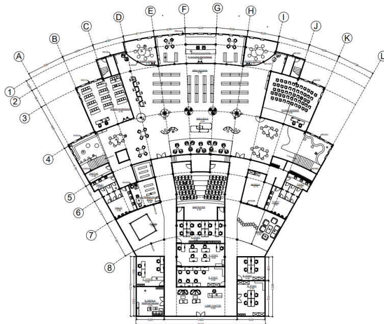
Gambar 3. Layout Lantai B1
