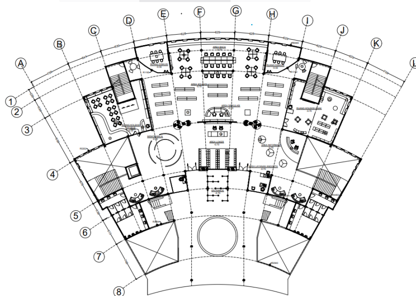
Gambar 2. Layout Lantai 1
