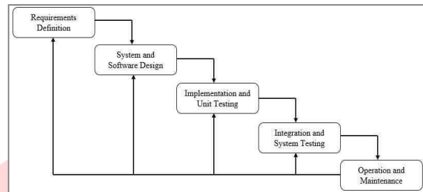
Gambar 1 Model Waterfall
