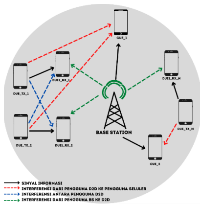
Gambar 1. Model Sistem
