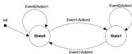
GAMBAR 2.1 DIAGRAM FINITE STATE MACHINE
