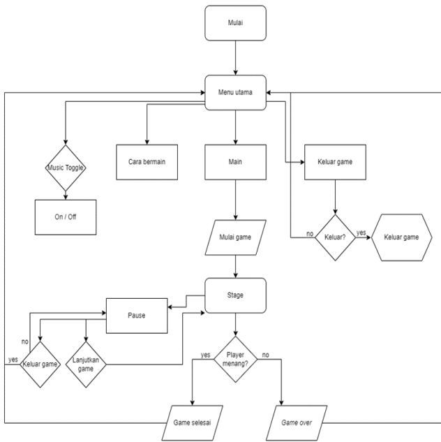
GAMBAR 3.1 FLOWCHART SISTEM
