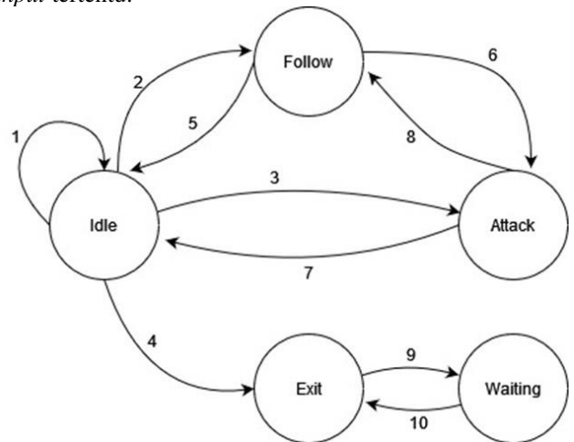
GAMBAR 3.3 DIAGRAM STATE NPC ERIC
