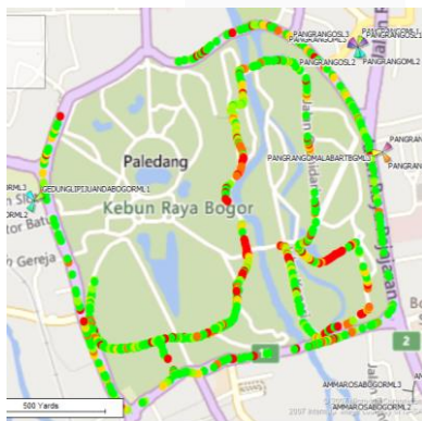
Gambar 6 Data BLER hasil drive test
