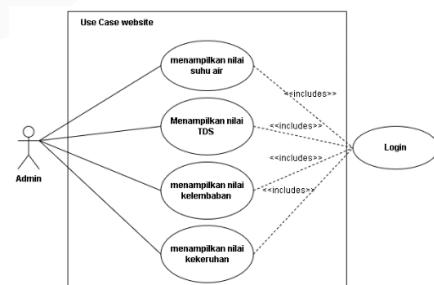
GAMBAR 3.5 USE CASE DIAGRAM
