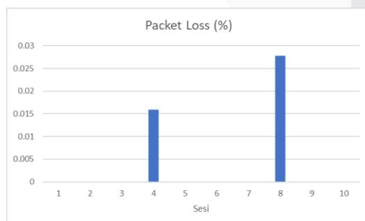
GAMBAR 4.6 HASIL PENGUJIAN PACKET LOSS
