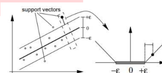
GAMBAR 2.2 FUNGSI SUPPORT VECTOR REGRESSION [11]
