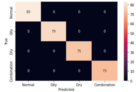
GAMBAR 3.5 CONFUSION MATRIX
