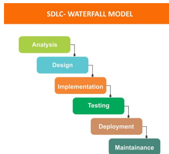
Gambar 1. 1 Model Waterfall/SDLC
