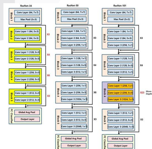
GAMBAR 2. Struktur layer ResNet-34, ResNet-50, ResNet-101
