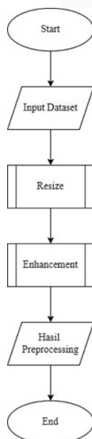
GAMBAR 3. Flowchart preprocessing
