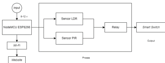
GAMBAR 2. Blok Diagram
