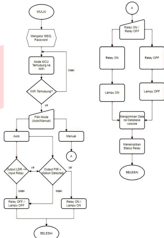
GAMBAR 3. Diagram Alir
