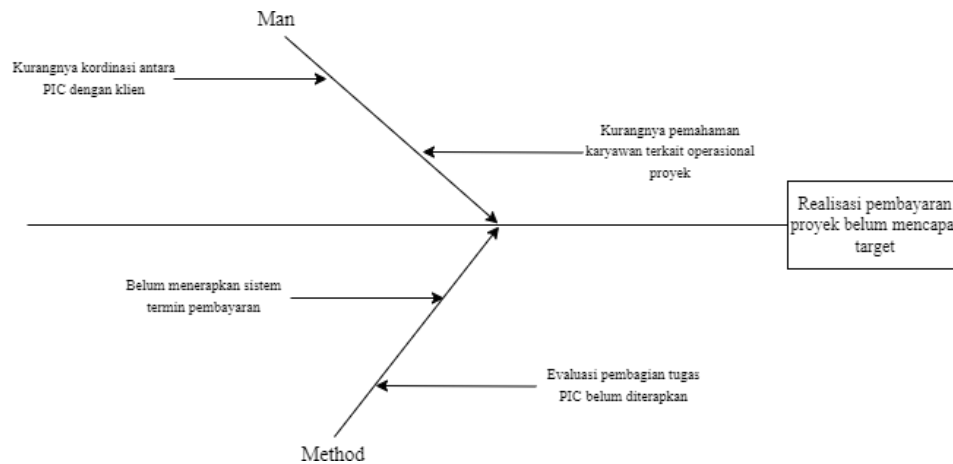
Gambar I. 2 Diagram Fishbone
